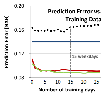
Figure 10. Prediction error as a function of days of training data from one stations per cluster at PW=120
